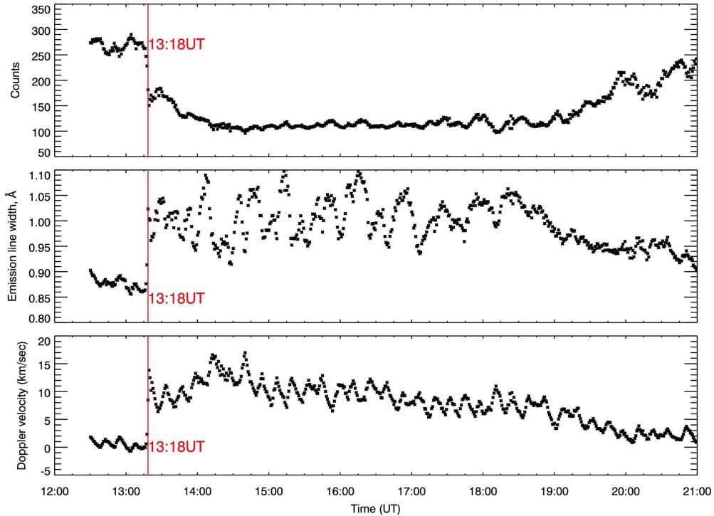
Fig. 7.— Upper panel: Time variation of the peak intensity of the emission line averaged over the dimming region (position angle range \approx 260^\circ - 270^\circ ) in Figure 3. The vertical red line indicates the onset of the dimming at \approx 13:18 UT. Middle panel: Same as above, but corresponds to width of the emission line. Lower panel: Same as above, but corresponds to Doppler velocity estimated from the shift in the peak of the emission line from the reference.
