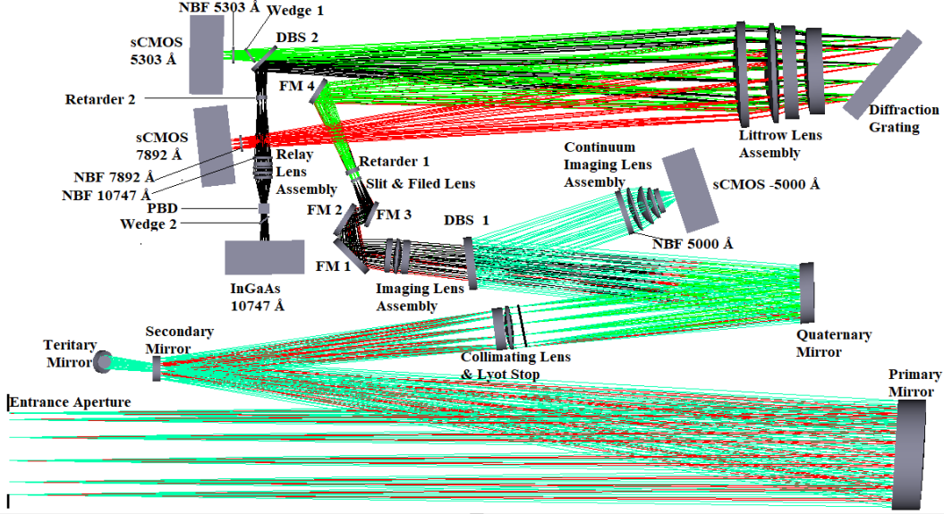
Fig. 1.— Optical layout of VELC
