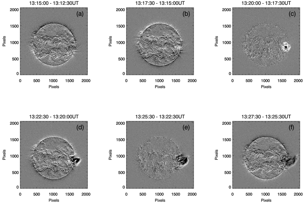
Fig. 4.— STEREO-A/EUVI 195Å running difference images for the flare event of 16 July 2024 mentioned in the text. The observing times of the images used are mentioned above each panel.
