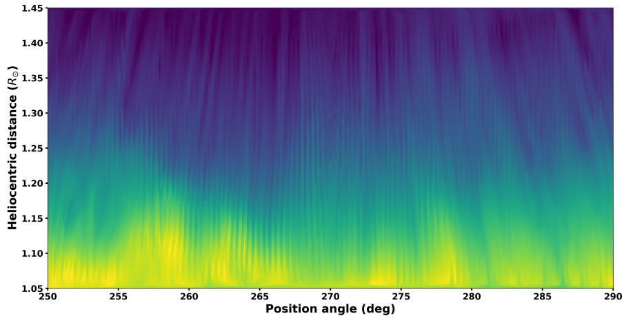
Fig. 6.— Same as Figure 5, but during the interval \approx 23:09 UT - 23:56 UT.
