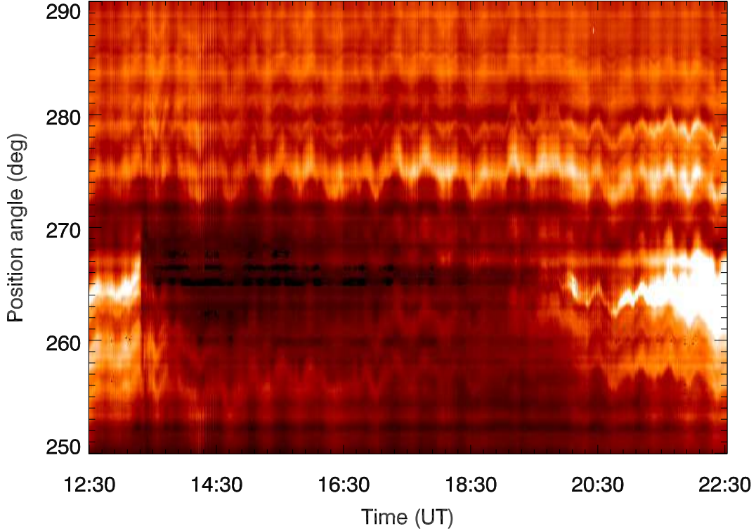
Fig. 3.— Temporal variations in the peak intensities of the 5303Å emission line from the solar corona in the position angle range \approx 250^\circ - 290^\circ observed on 16 July 2024 with VELC/ADITYA-L1. The center of spectrograph slit 4 was positioned close to the west limb of Sun at r \approx 1.05 R_\odot . A sudden dimming of the intensity can be clearly observed in the position angle range \approx 260^\circ - 270^\circ during the interval \approx 13:18 UT - 19:00 UT. The possible reasons for the oscillatory pattern in the image are being investigated.
