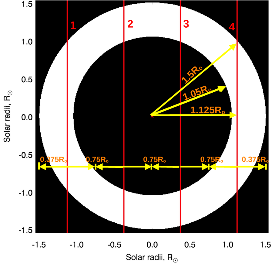
Fig. 2.— Schematic of the ‘home’ positions of the four slits in the VELC spectroscopy channel. The inner filled black circle corresponds to the occulter (radius = 1.05 R_{\odot} ). The white circular patch indicates the FoV, i.e. 1.05 R_{\odot} - 1.5 R_{\odot} . Solar north and east directions are straight up and to the left, respectively.
