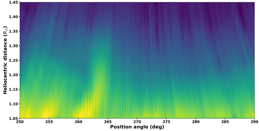
Fig. 5.— (r, \theta) image of the solar corona at west limb of Sun constructed from the raster scan observations in 5303\text{\AA} emission line on 16 July 2024 during the interval \approx 00:30 UT - 01:17 UT, with VELC/ADITYA-L1. The fine lines seen in the image are due to remnant fixed pattern noise due to the detector, even after the flat field correction.
